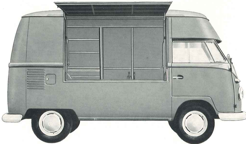
The VW Mobile Shop with raised roof Sales flap: height 40.2 inches, width 64.4 inches Height from ground to lower edge of sales flap: approx. 41.3 inches Height of sales room: 68.9 inches
